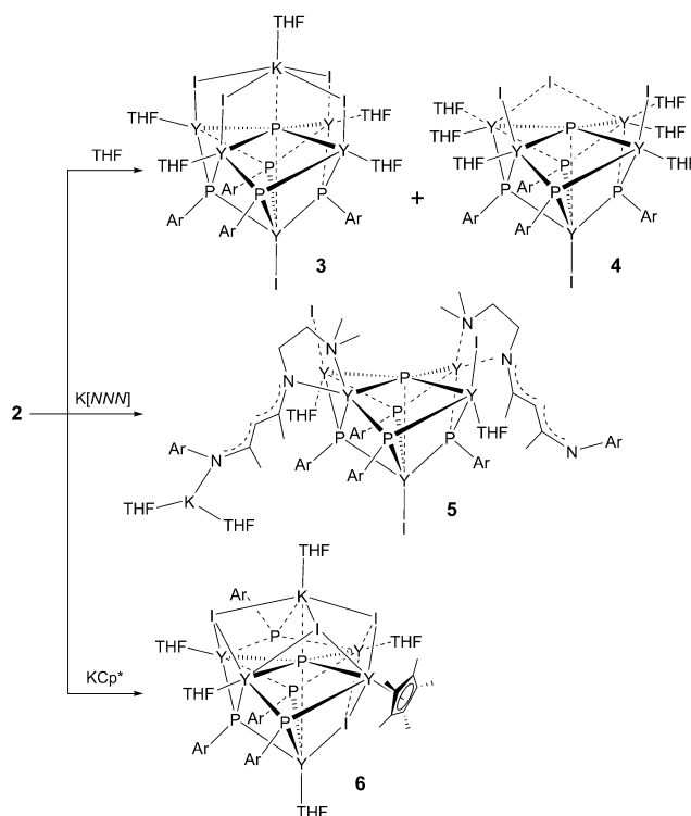
Scheme 2. Syntheses of 3 – 6 .
