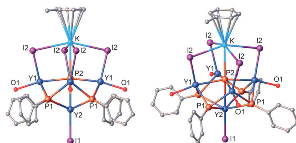
Figure 1. Two views of molecular structure of 2 . Isopropyl groups on the Ar rings, hydrocarbon fragments of thf molecules, all hydrogen atoms, and solvents in the lattice are omitted for clarity.
