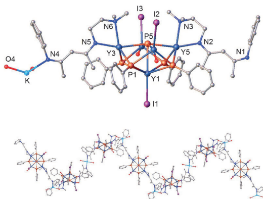
Figure 3. Molecular structure of 5 . Isopropyl groups on the Ar rings, hydrocarbon fragments of thf molecules, all hydrogen atoms, and solvents in the lattice are omitted for clarity.
